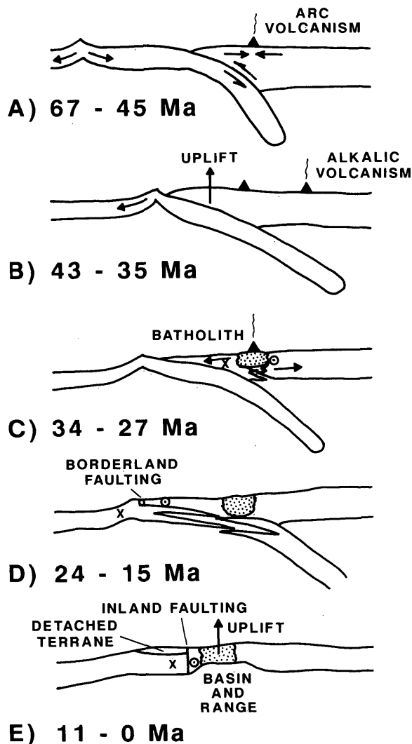
Fig 9. A model of the interaction of a mid-ocean ridge with a trench where the ridge strikes at a high angle to the trench. See description in text. Shear parallel to the trench is shown by dots (tips of arrows) and crosses (tails of arrows).
